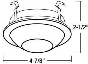
Trim OD: 4-7/8" Height: 2-1/2"
