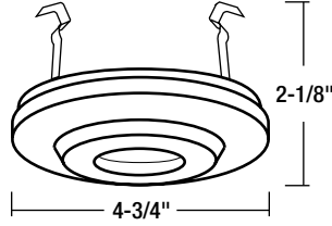
Trim OD: 4-3/4" Height: 2-1/8"
