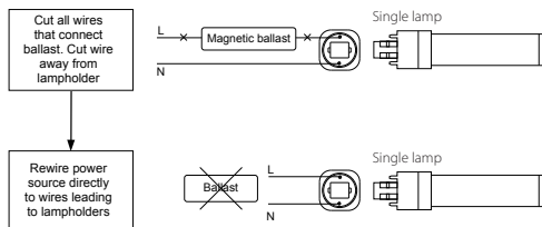
Diagram 2 – Magnetic ballast fixture wiring modification
