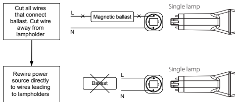
Diagram 2 – Magnetic ballast fixture wiring modification
