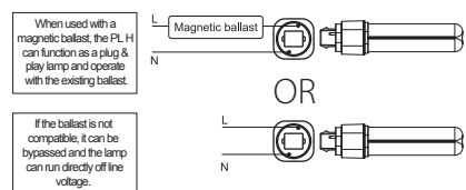
Diagram 3 – Magnetic ballast fixture wiring modification
