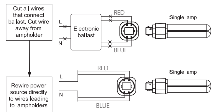
Diagram 2 – Electronic ballast fixture wiring modification
