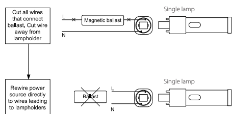
Diagram 3 – Magnetic ballast fixture wiring modification
