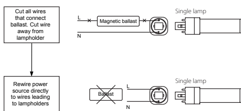
Diagram 2 – Magnetic ballast fixture wiring modification
