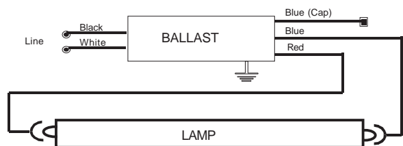
ONE LAMP APPLICATION Cap any blue lead, insulate to 800 volts
