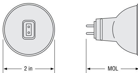
GU5.3 Base
